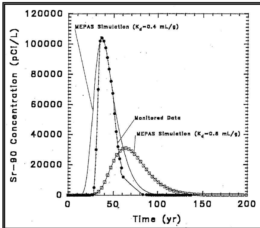
Figure 4.3. Example illustrating MEPAS 90 Sr calibrations with K_d equaling 0.4 and 0.8 ml/g and several monitored-data points.
